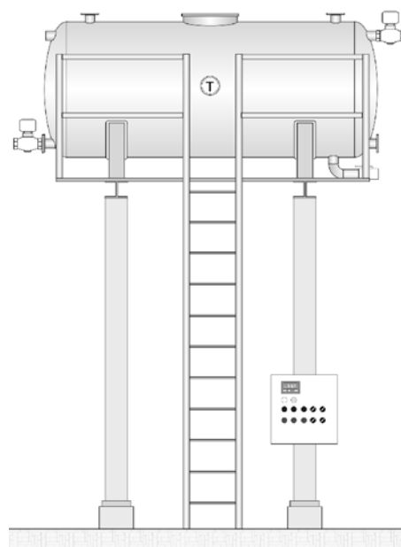
OPTIONAL SUPPORT TRELLIS
