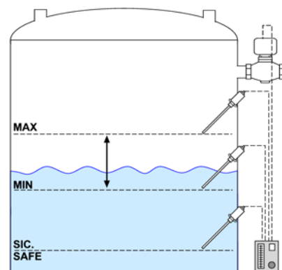
WATER-LEVEL CONTROL
